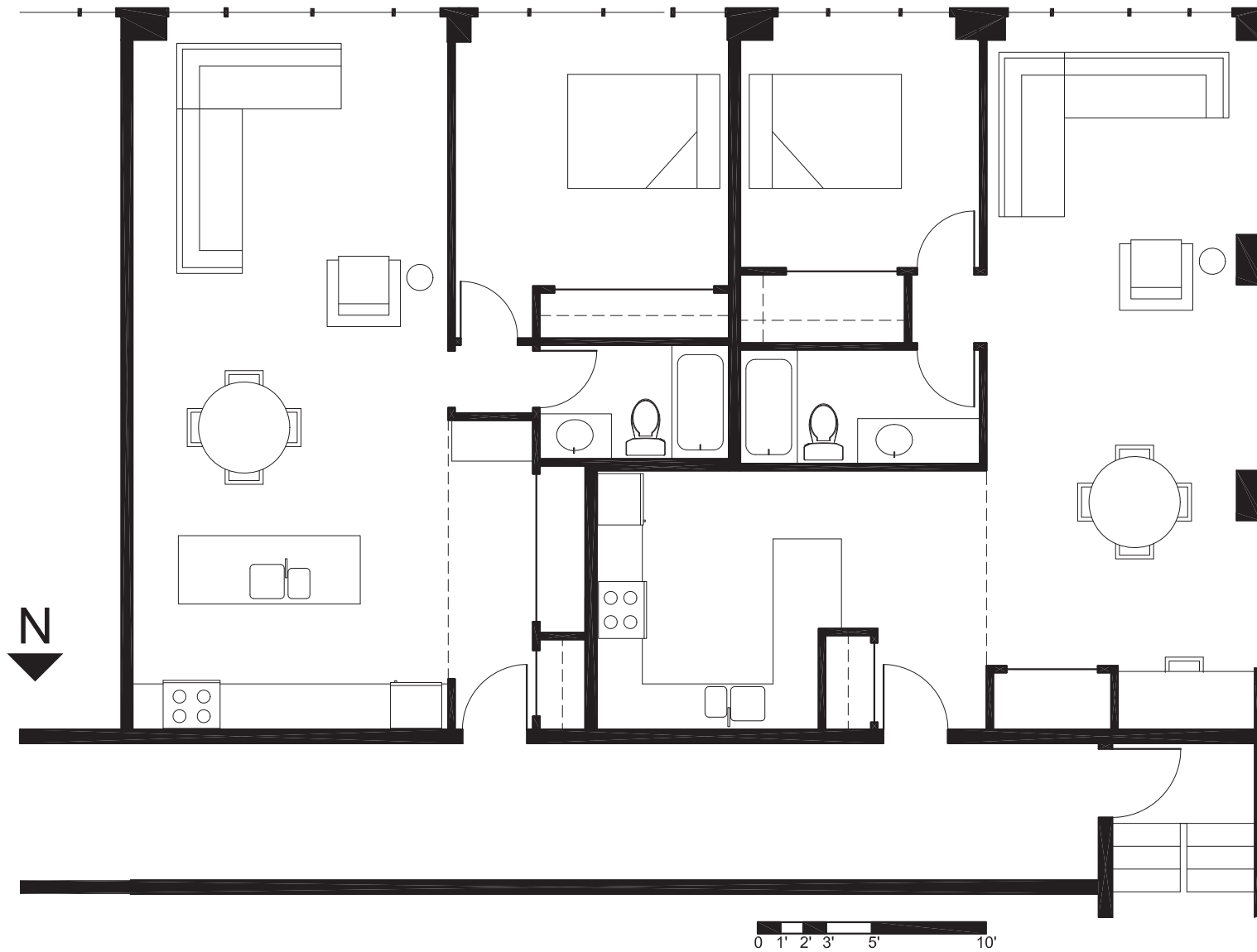
This is the final floor plan for the completed concept design, including furniture, for this week's Design Project.
